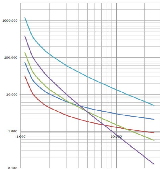
IEC/IEEE Inverse curves for tripping of over current elements
