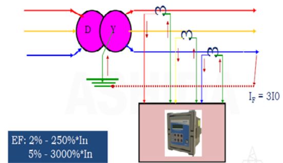
Internally derived residual over current application
